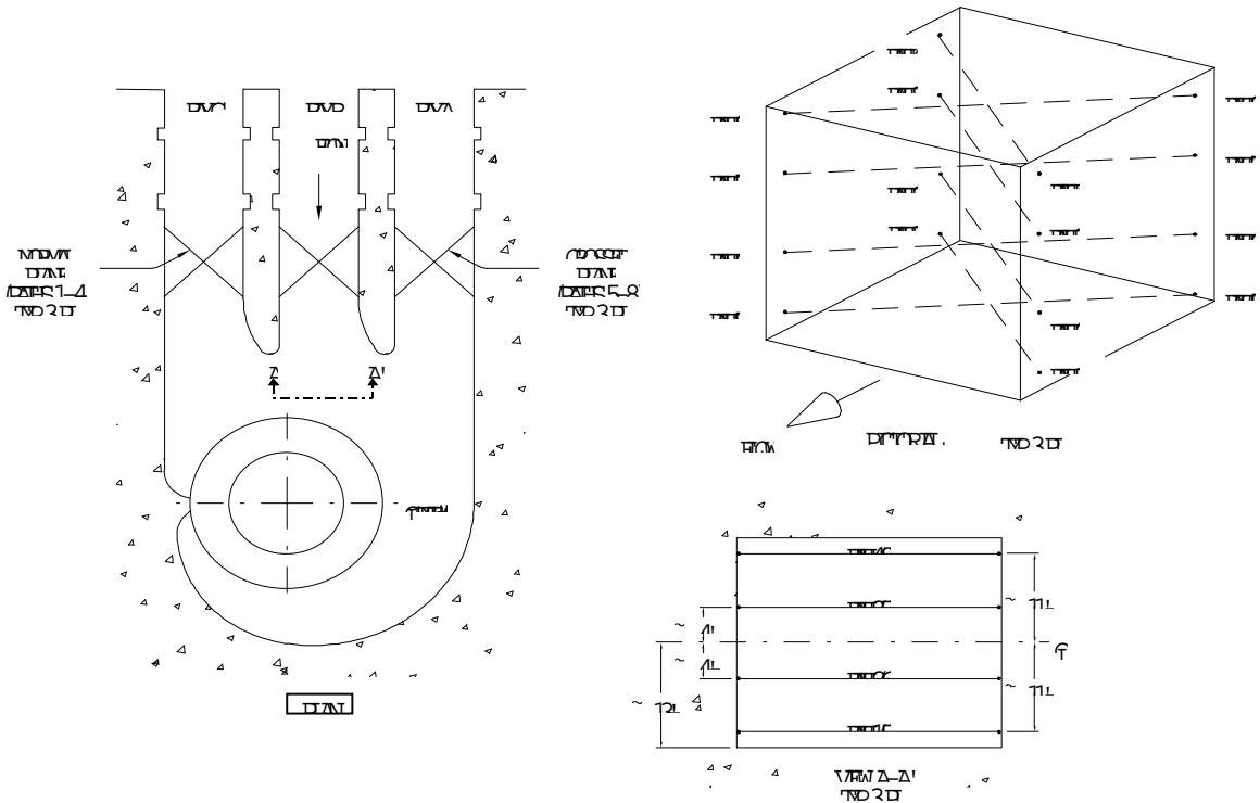
Figure 3. Ultrasonic flowmeter acoustic-path arrangement for a low-head 3-bay intake configuration.
