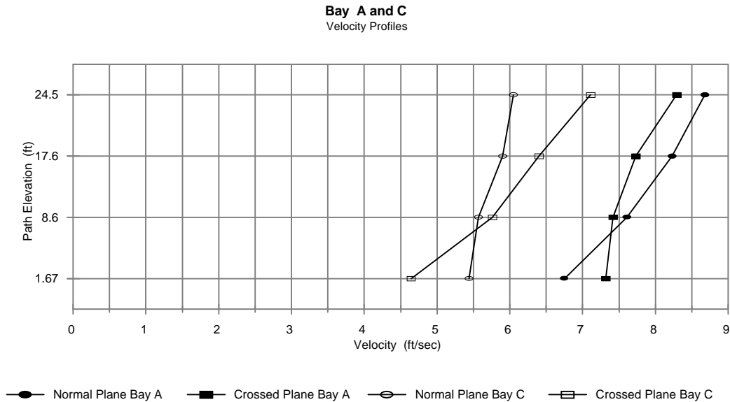
Figure 4. Typical velocity profile in 2 of 3 bays for one flowrate run.
